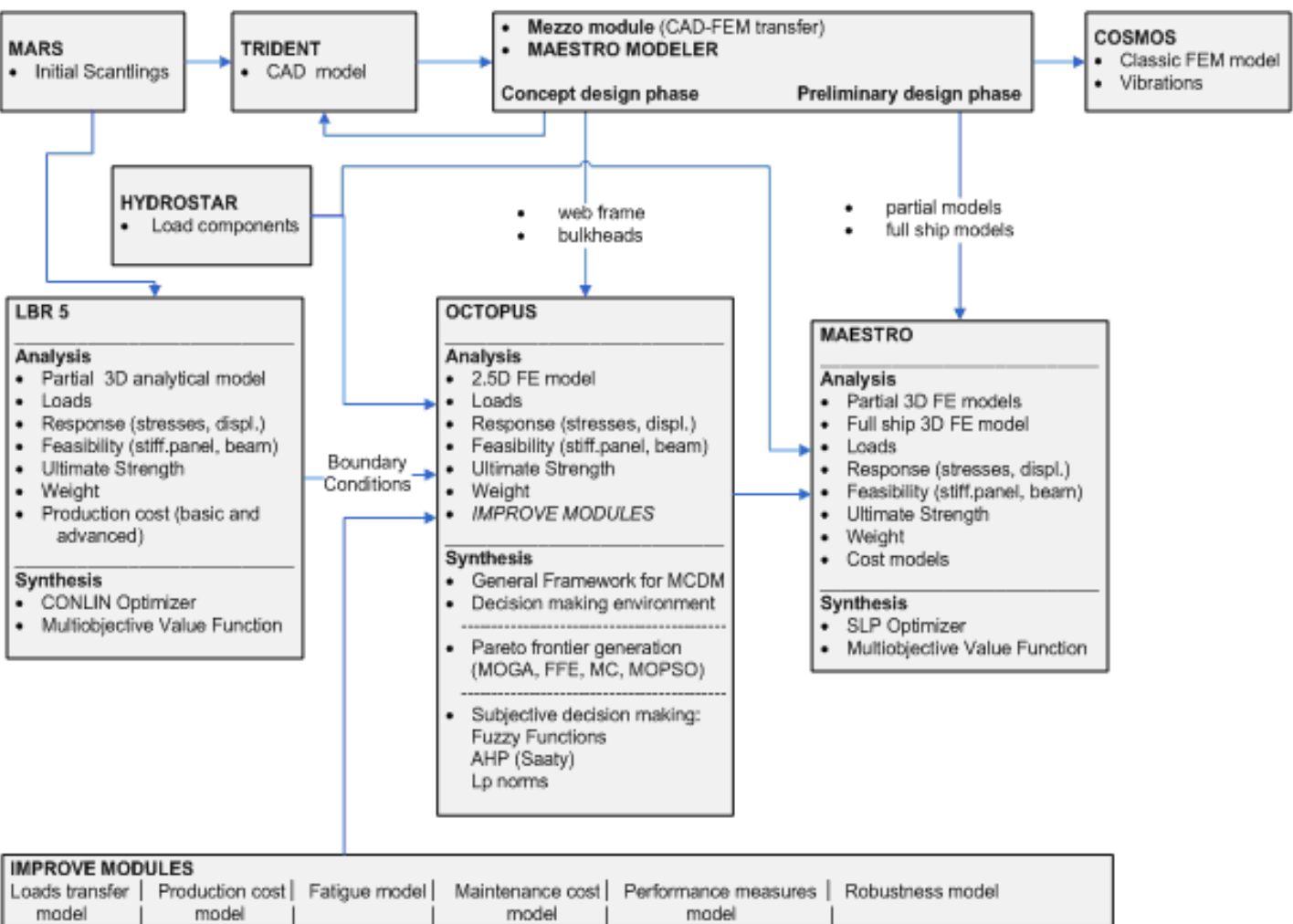
Overall structural design flowchart
