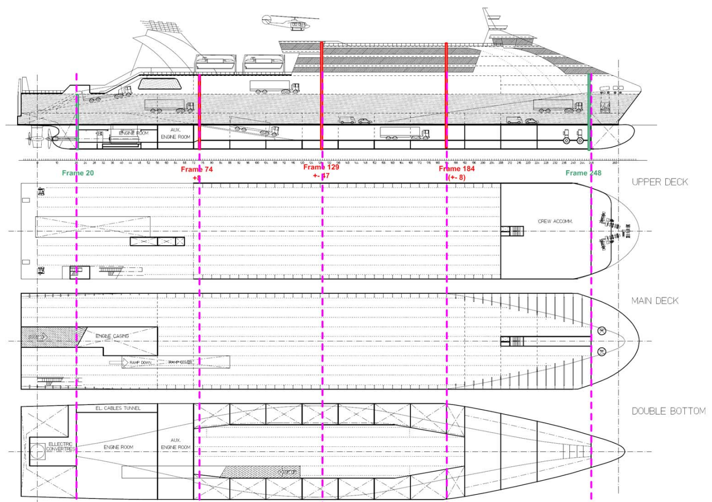
General Arrangement of the RoPax Design
